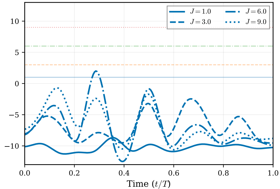
(b) Adapted ZZ Coupling Pulses
