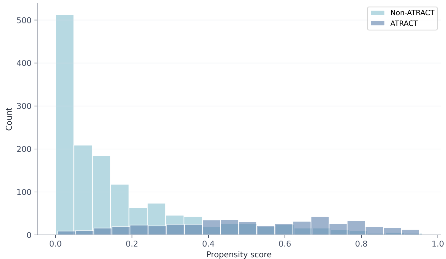
Propensity score overlap in the supported speed cohort
