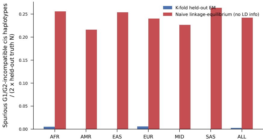
Non-circular mask-and-rephase: held-out EM vs. no-LD-information baseline
