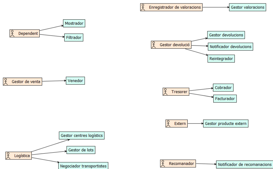
Fig. 23: Agent-Role Grouping
