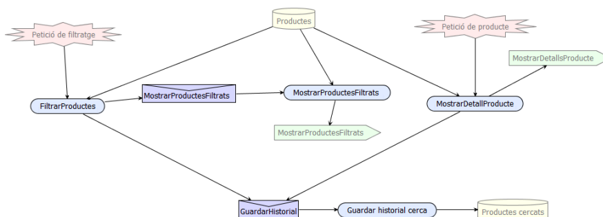
Fig. 33 Plans Dependent Agent
