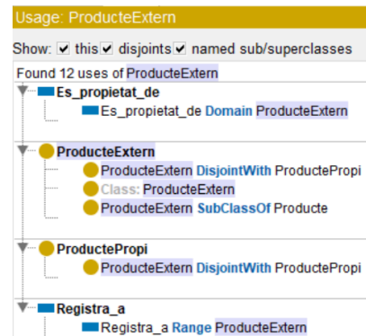
Fig. 66 Usage ProducteExtern
