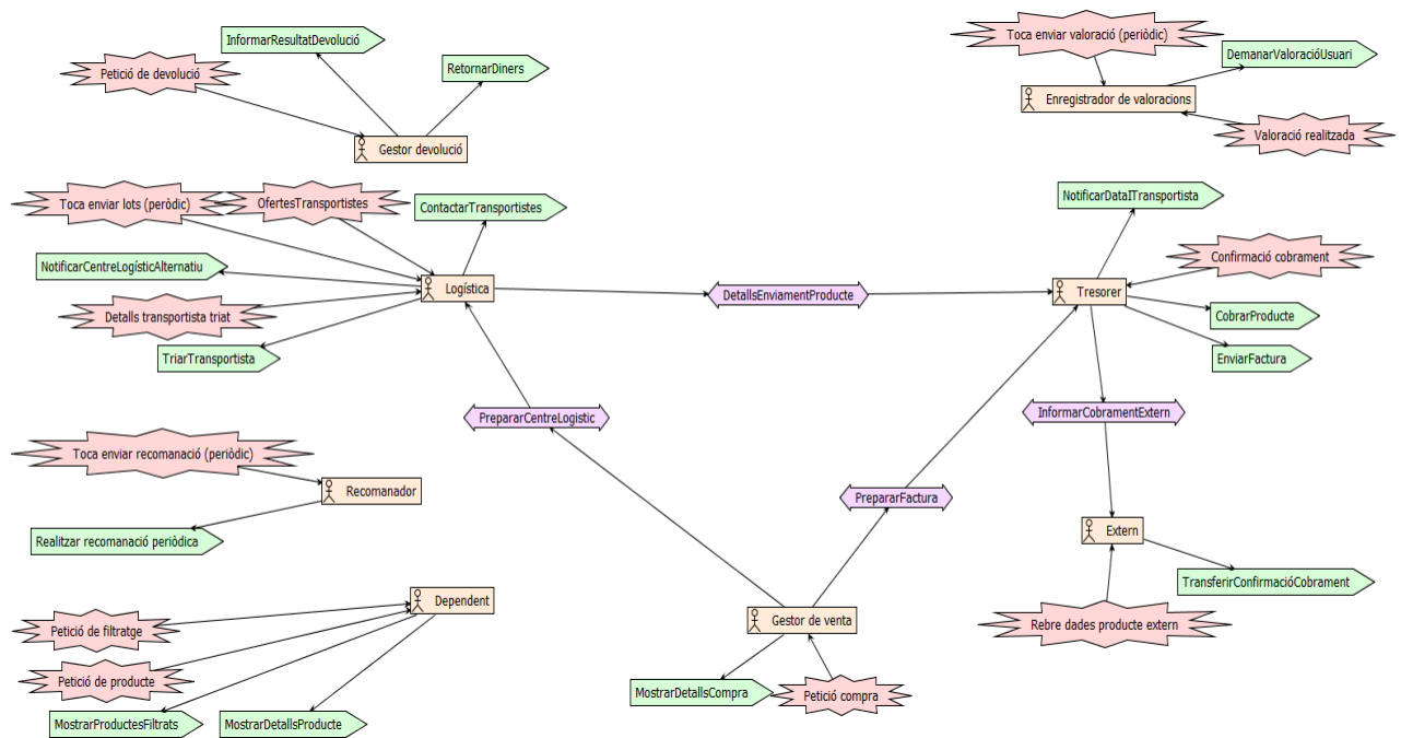
Fig. 25 System Overview
