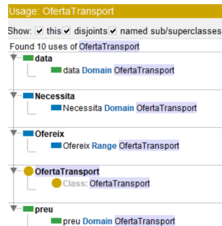
Fig. 64 Usage OfertaTransport
