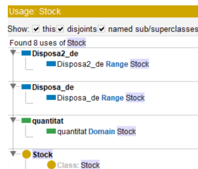
Fig. 68 Usage Stock
