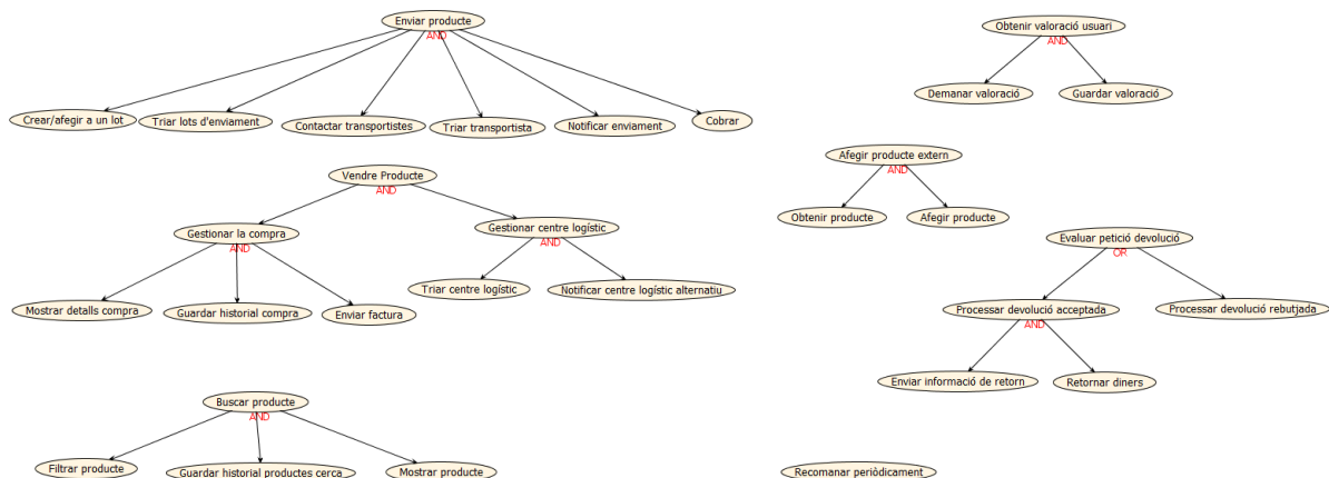
Fig. 13 Goal Overview
