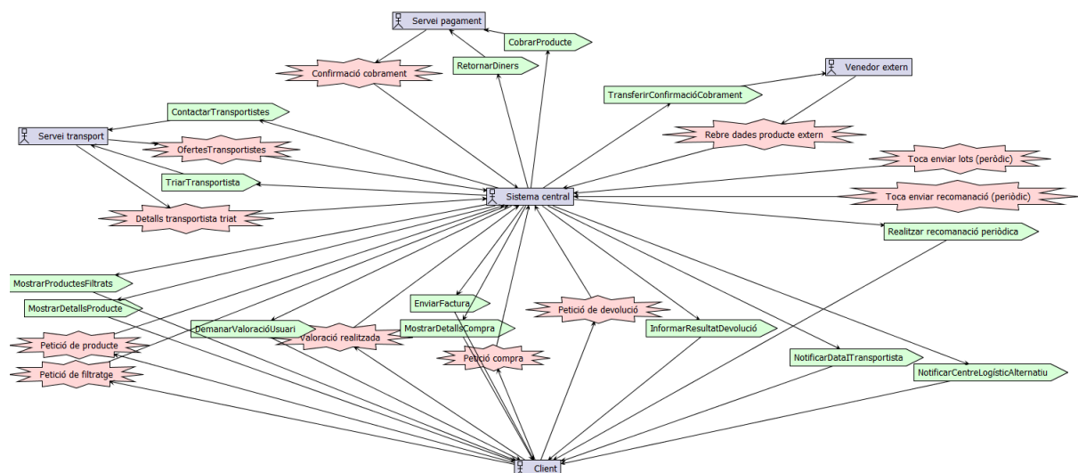
Fig. 1 Analysis Overview
