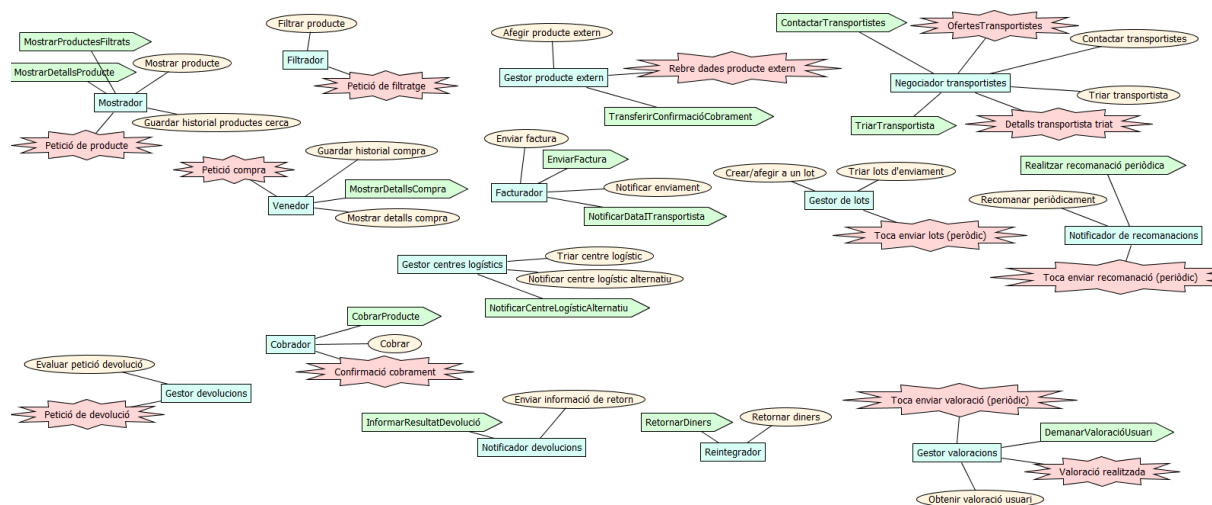
Fig. 21 System Roles
