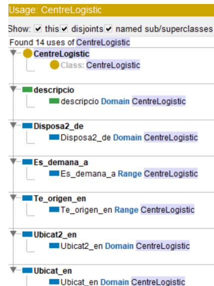
Fig. 56 Usage CentreLogistic
