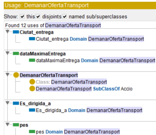
Fig. 49 Usage DemanarOfertaTransport
