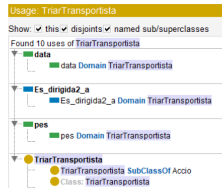
Fig. 55 Usage TriarTransportista
