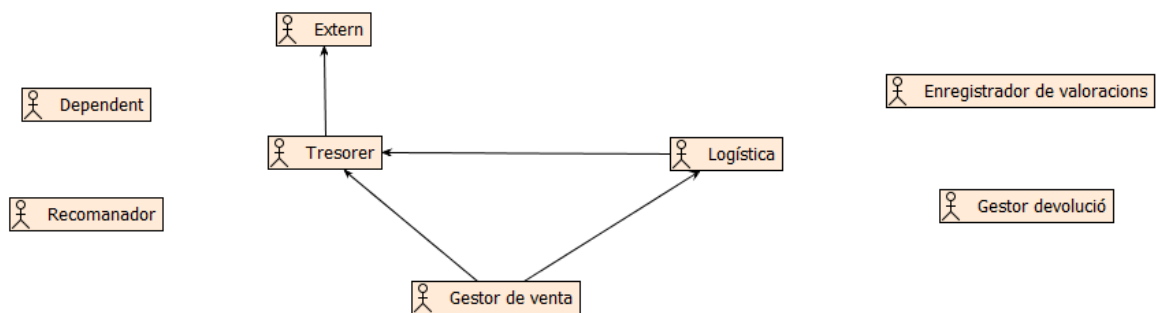
Fig. 24 Agent Acquaintance
