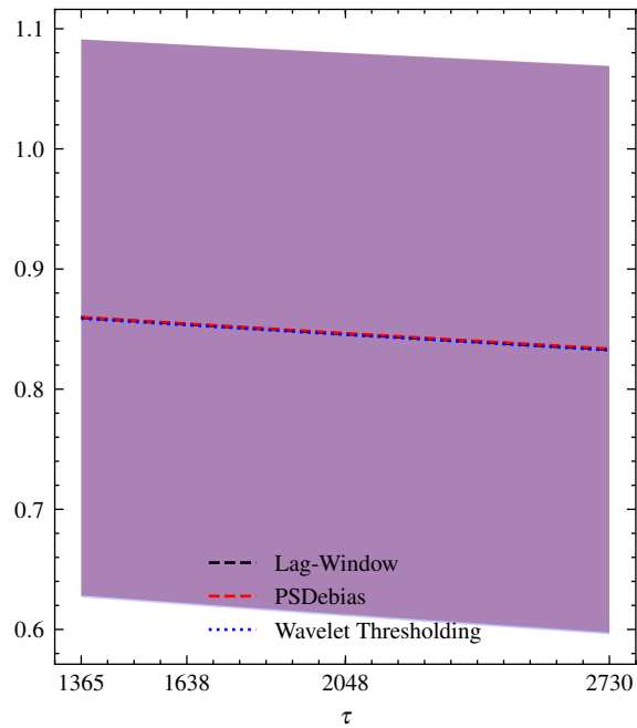
Bias
