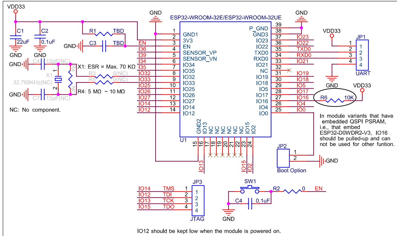
Figure 8: Peripheral Schematics
