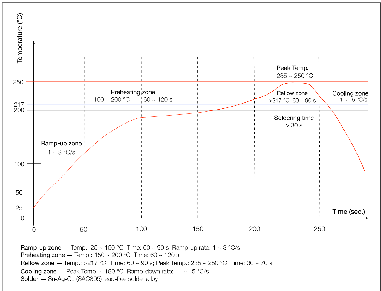
Figure 14: Reflow Profile
