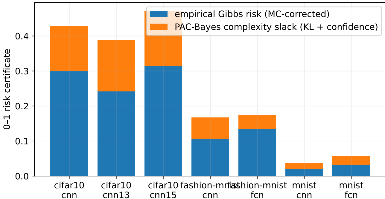
Certificate anatomy (fquad, learnt prior, full data)
