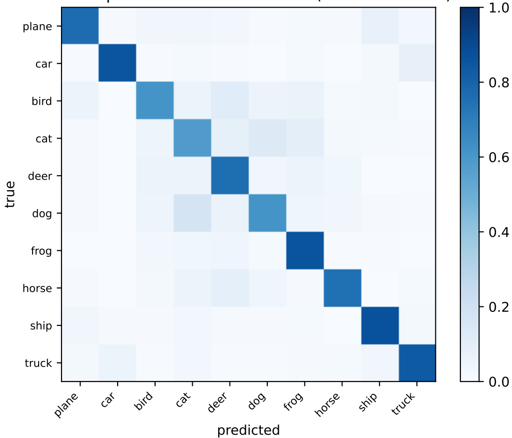
cifar10 posterior-mean confusion (row-normalised)
