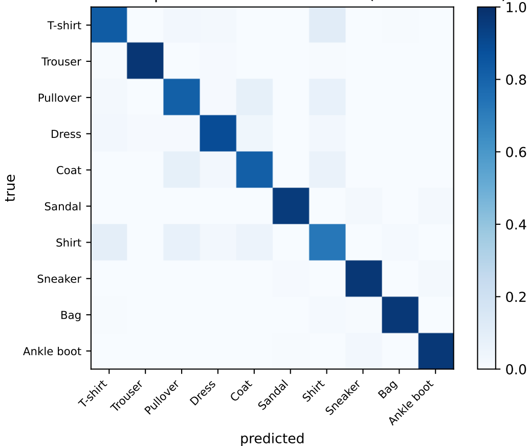
fashion-mnist posterior-mean confusion (row-normalised)
