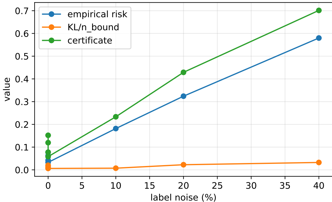
Controlled difficulty (same arch / data size, MNIST FCN)
