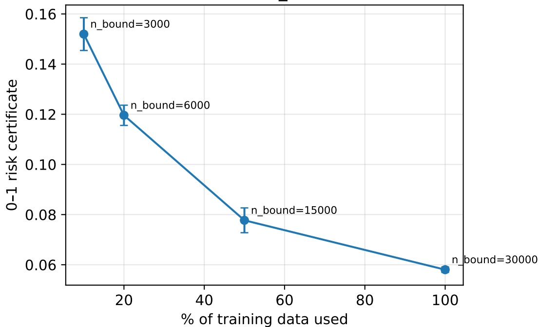
Small-data certificate (corrected n_{\text{bound}} , error bars over seeds)
