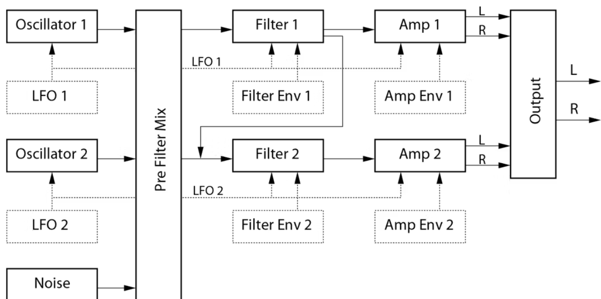
Diagram of Analog's Signal Flow.
