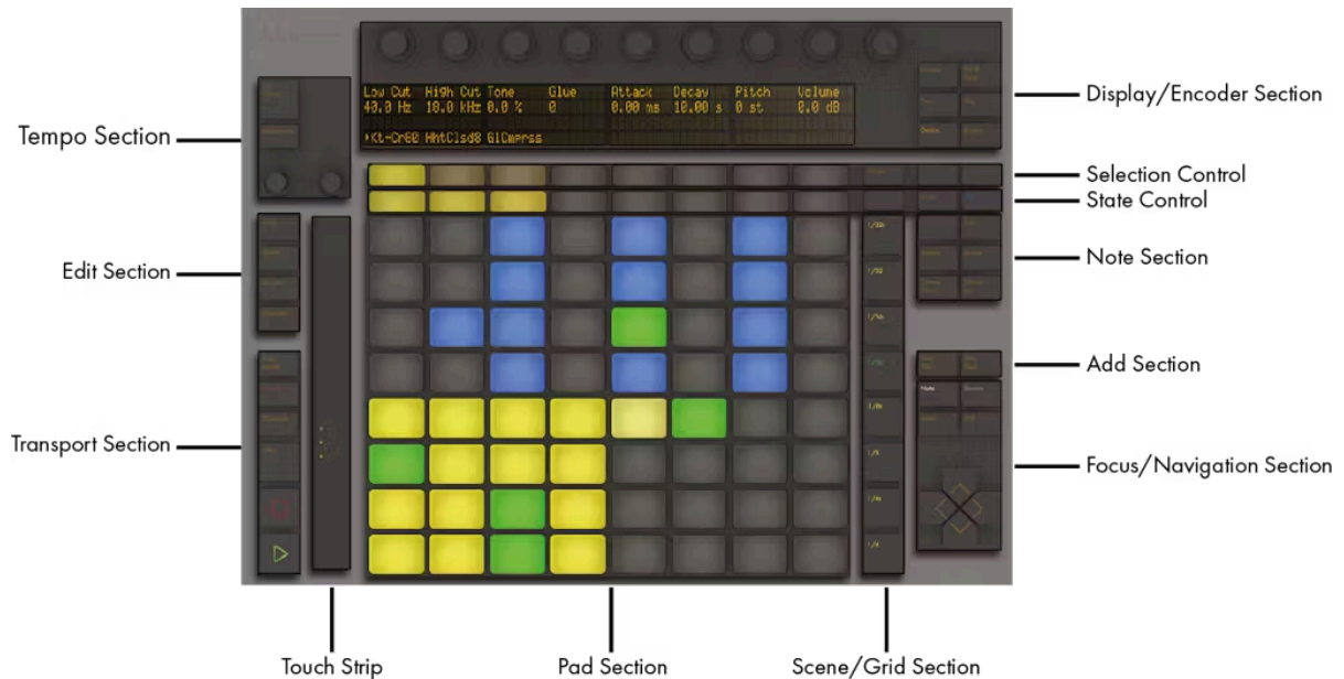
Overview of Push 1's Controls.
