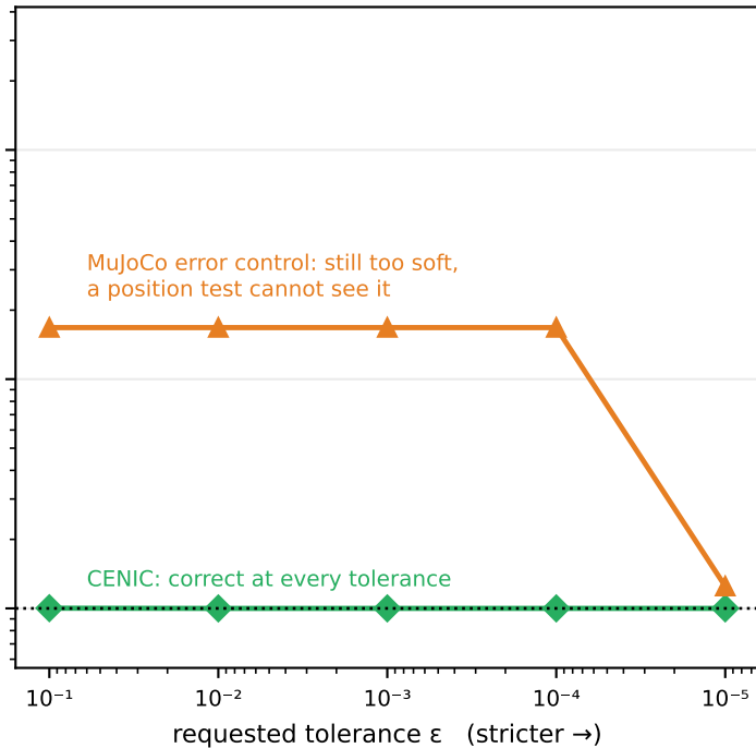
(b) Error control: asking for more accuracy \rightarrow
