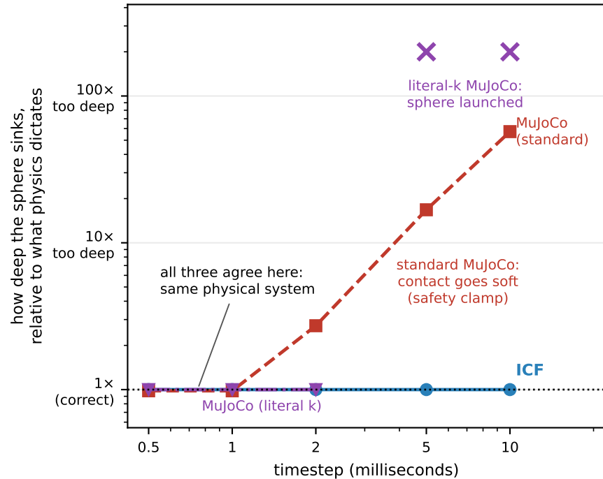
(a) Fixed timestep: coarser \rightarrow
