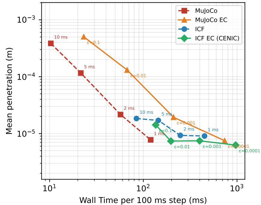
Hard Clutter
