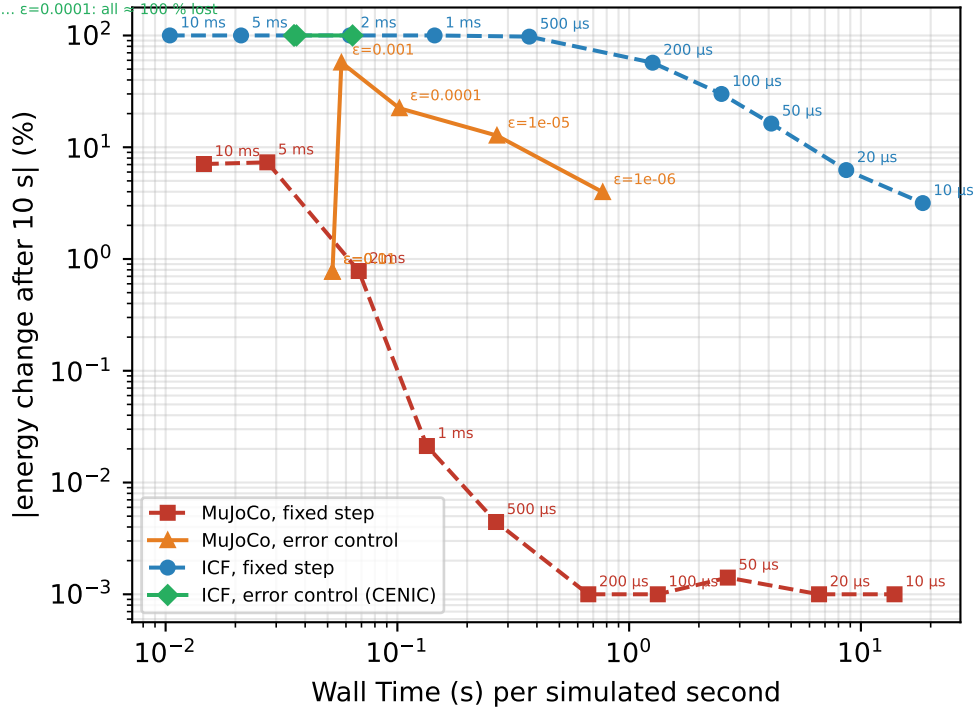
Bouncing ball — energy error vs cost
