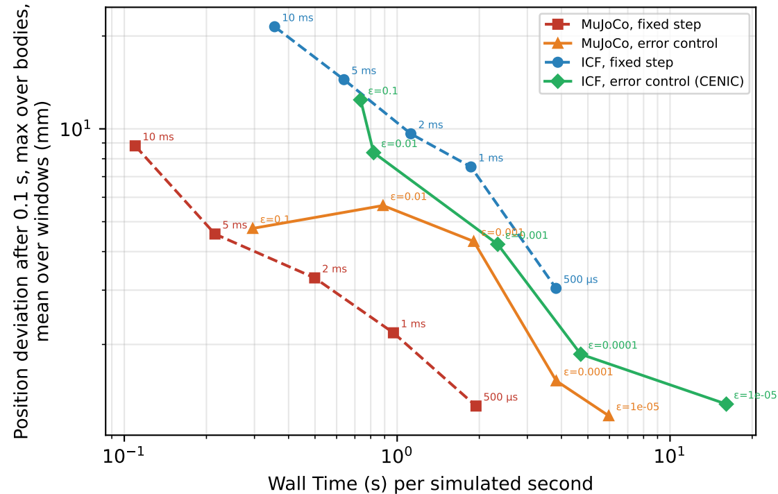
Hard Clutter — measured error vs cost (reference \delta t = 0.1 ms, same model)
