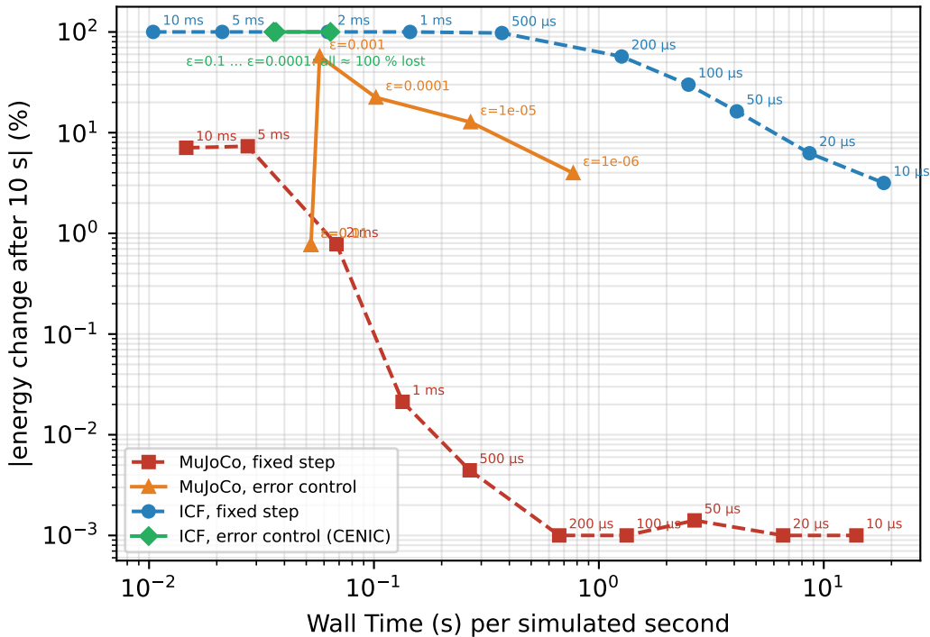
Bouncing ball — energy error vs cost
