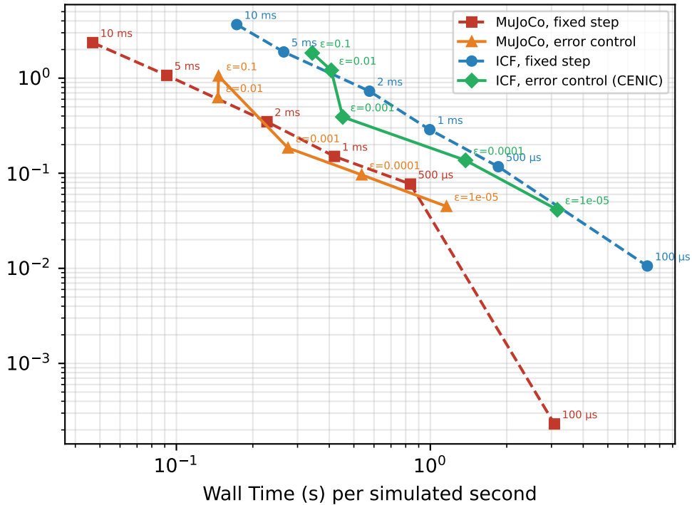
Soft Clutter — measured error vs cost (reference \delta t = 0.1 ms, same model)
