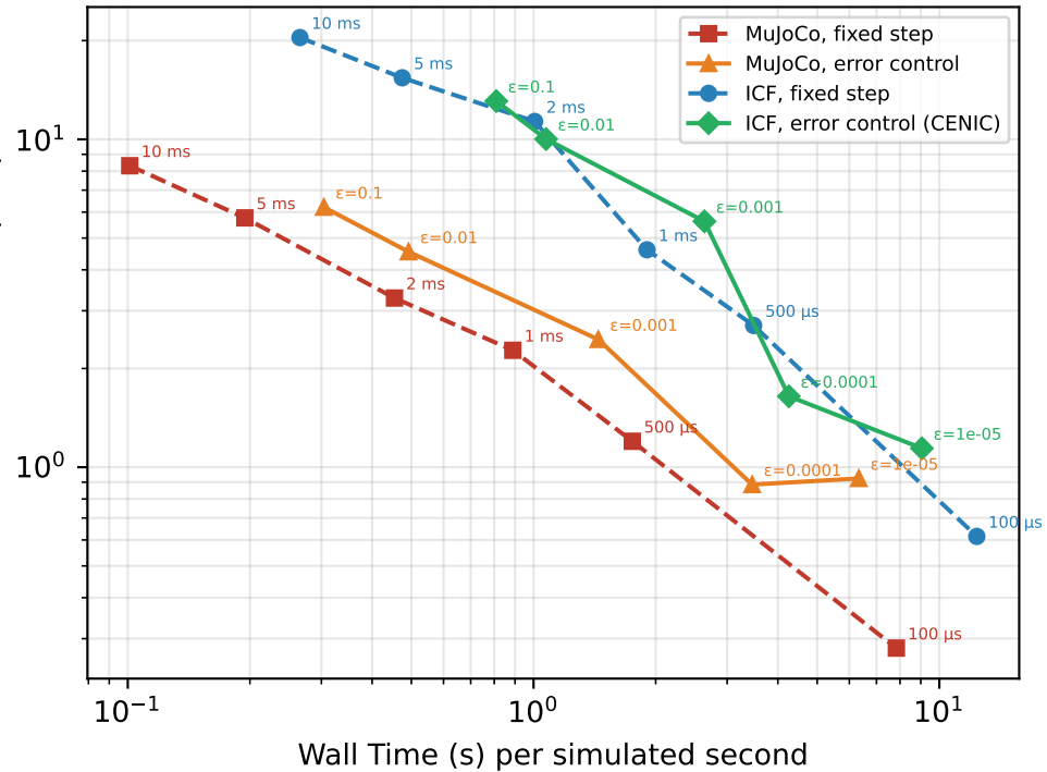
Hard Clutter — measured error vs cost (reference \delta t = 0.1 ms, same model)
