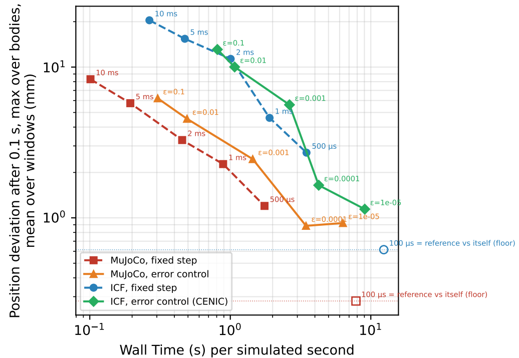
Hard Clutter — measured error vs cost (reference \delta t = 0.1 ms, same model)
