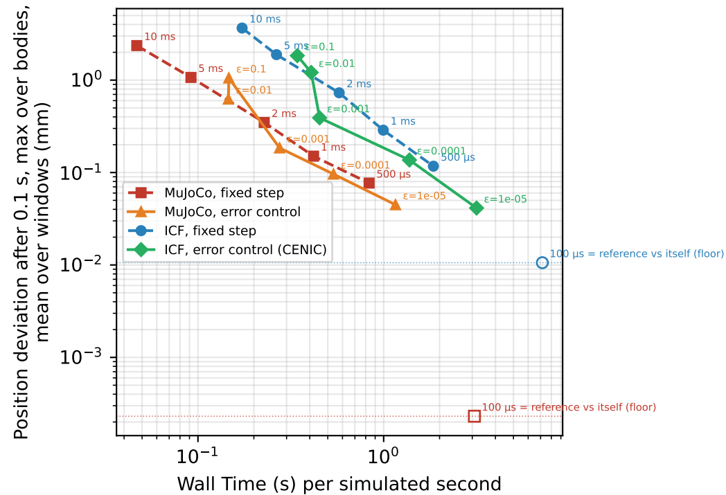
Soft Clutter — measured error vs cost (reference \delta t = 0.1 ms, same model)
