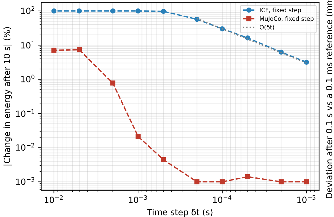
(a) Bouncing ball, zero dissipation: ICF converges at first order; MuJoCo's undamped soft constraint holds the energy within 0.03 % at \delta t \leq 1 ms
