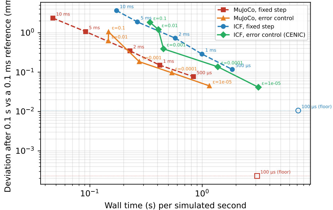
(b) Soft clutter, measured error vs cost: first order for both; ICF error control \sim 2\times less deviation than fixed ICF at the same cost; hollow = the reference vs itself
