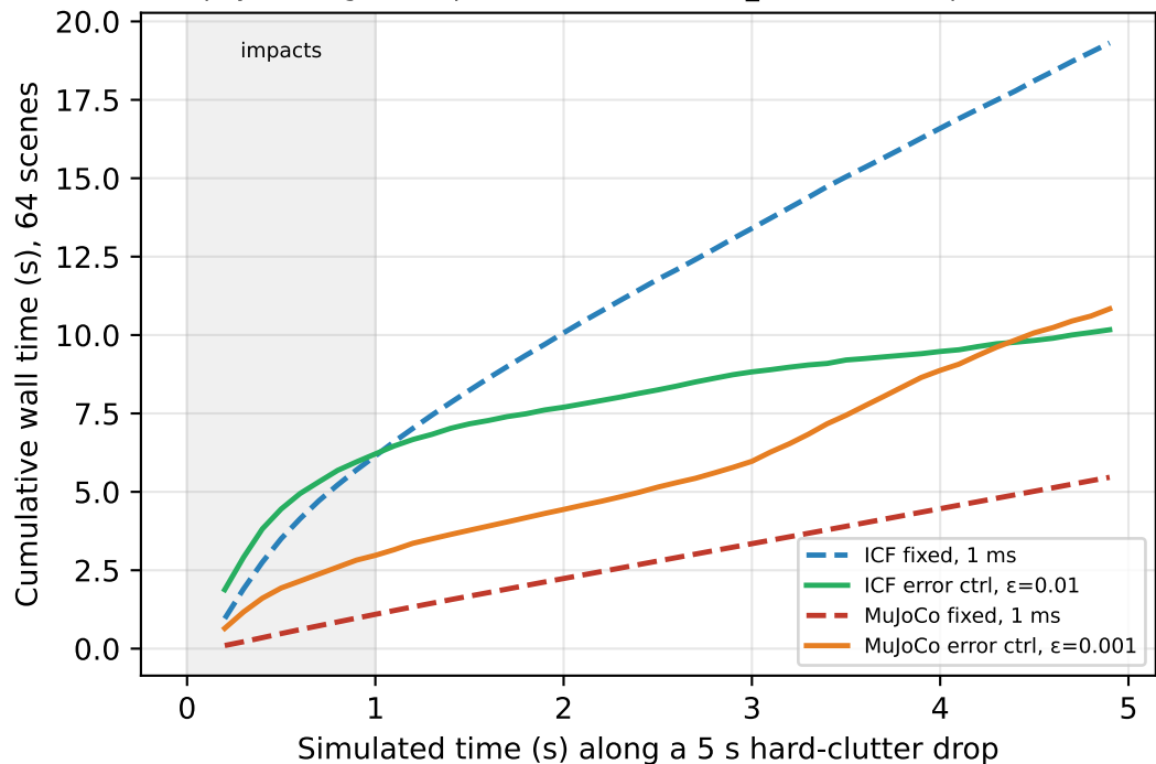
(b) Where the cost goes: fixed step pays the same every step; error control pays during the impacts and coasts at \delta t_{\max} once the pile settles
