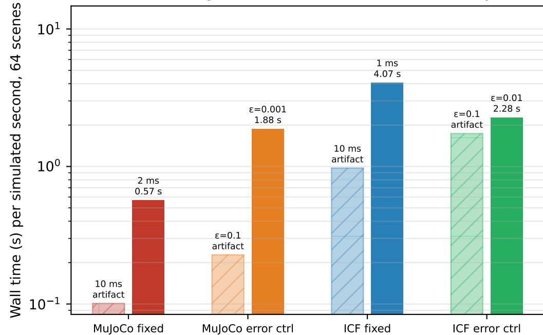
(a) Hard clutter: the learner's coarse setting (hatched, artifacts) vs the cheapest artifact-free setting of each arm (solid) — the matched-accuracy cost
