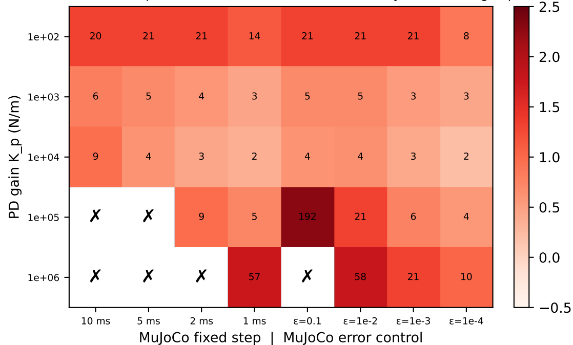
(c) A PD gantry pushing a 1 kg box: MuJoCo's box hops (mm) and its joint gain diverges (X) at the learner's steps; ICF: stable in all 40 cells, lift \leq 0 (stays at its resting depth)
