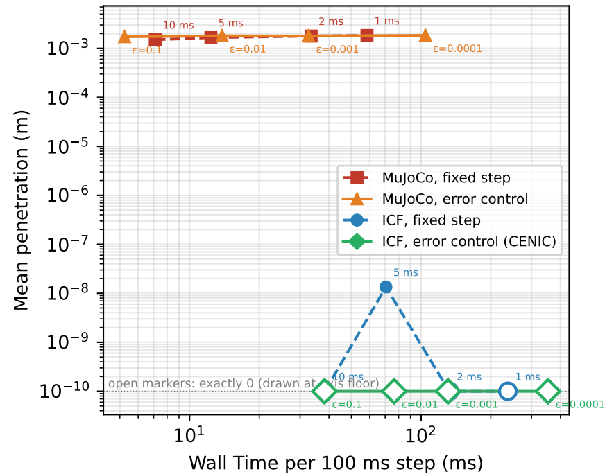
Soft Clutter, 64 worlds; 5 mm collision margin; no body left the bin in any configuration
