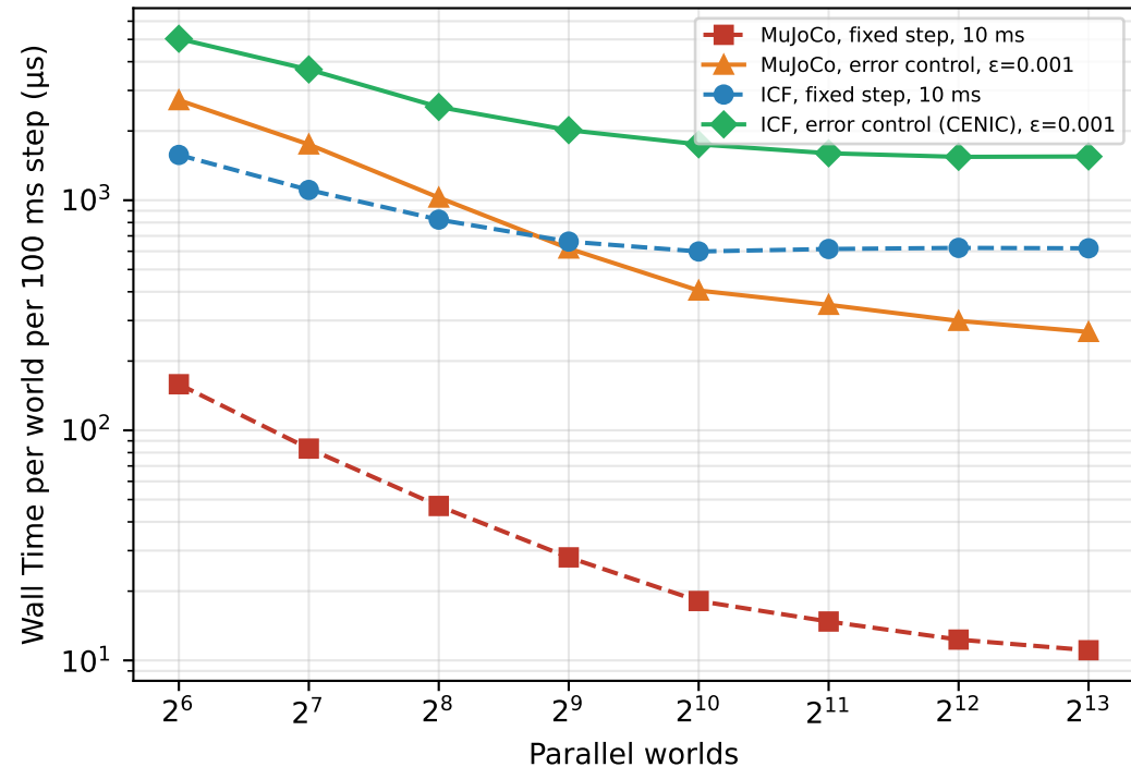
Hard Clutter — cost per world falls until the GPU saturates
