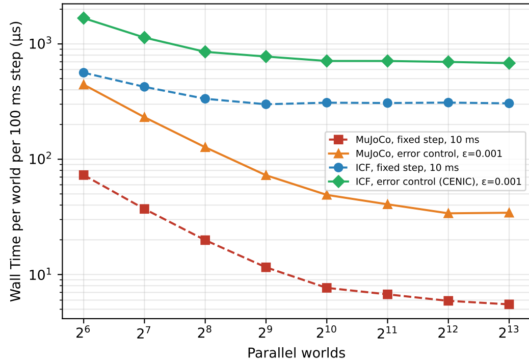
Soft Clutter — cost per world falls until the GPU saturates
