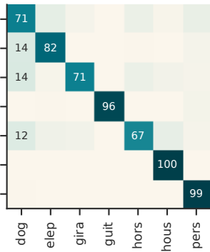
DANN (78.0%)
