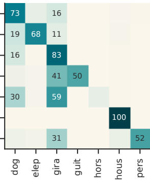
CDAN (56.8%)
