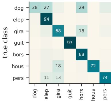
Source-only (74.2%)
