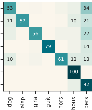
DAN (62.7%)
