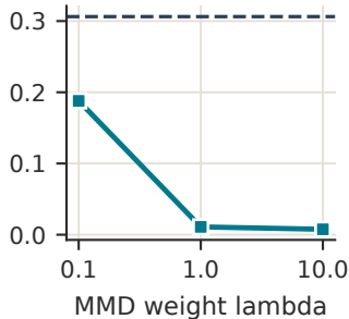
sharpness proxy
