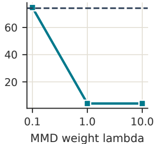
Sketch accuracy (%)
