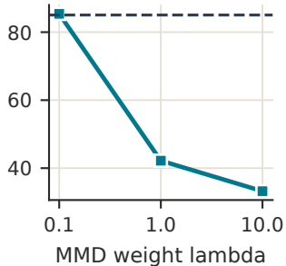
source separability (%)
