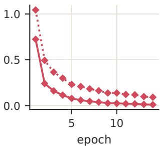
SAM: loss at theta (solid) and at theta+eps (dotted)
