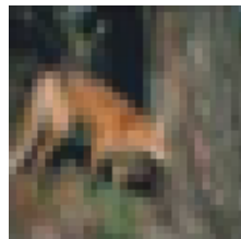
predicted deer MLS -11.15 (tau -5.79)
