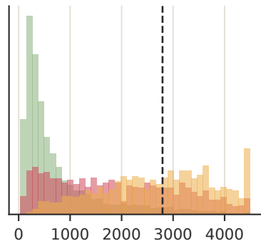
Mahalanobis: unknownness
