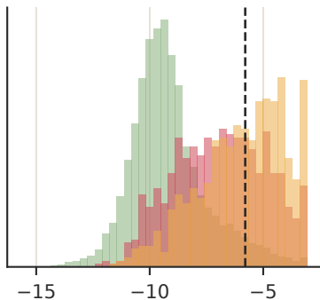
MLS: unknownness
