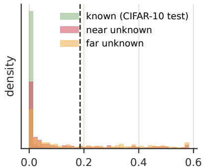
MSP: unknownness
