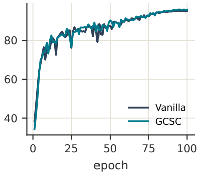
CIFAR-10 val accuracy (%)
