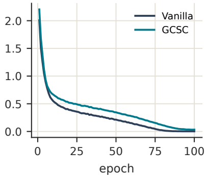
train loss (Vanilla, GCSC)
