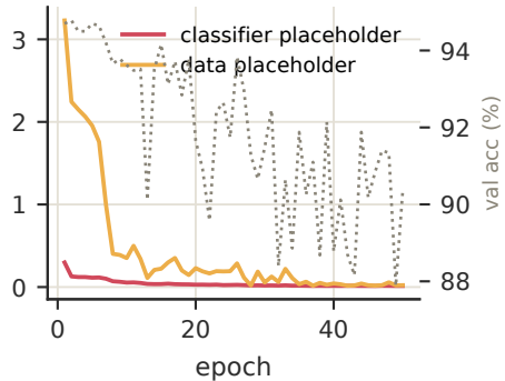
PROSER fine-tuning losses
