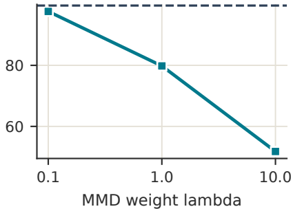
domain separability (%)
