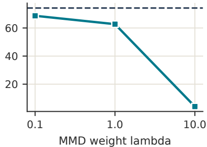
target accuracy (%)
