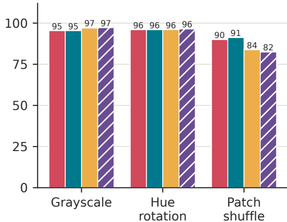
Prediction consistency vs clean (%)
