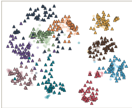
ResNet-50
