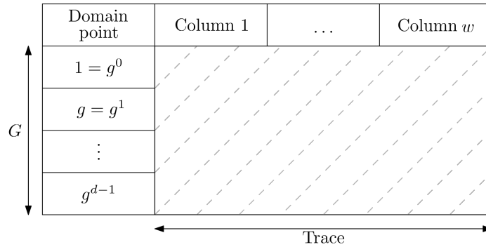
Figure 6: Trace representation
