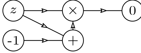
Figure 4: is_bool circuit
