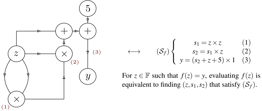
Figure 5: Circuit representation of f
