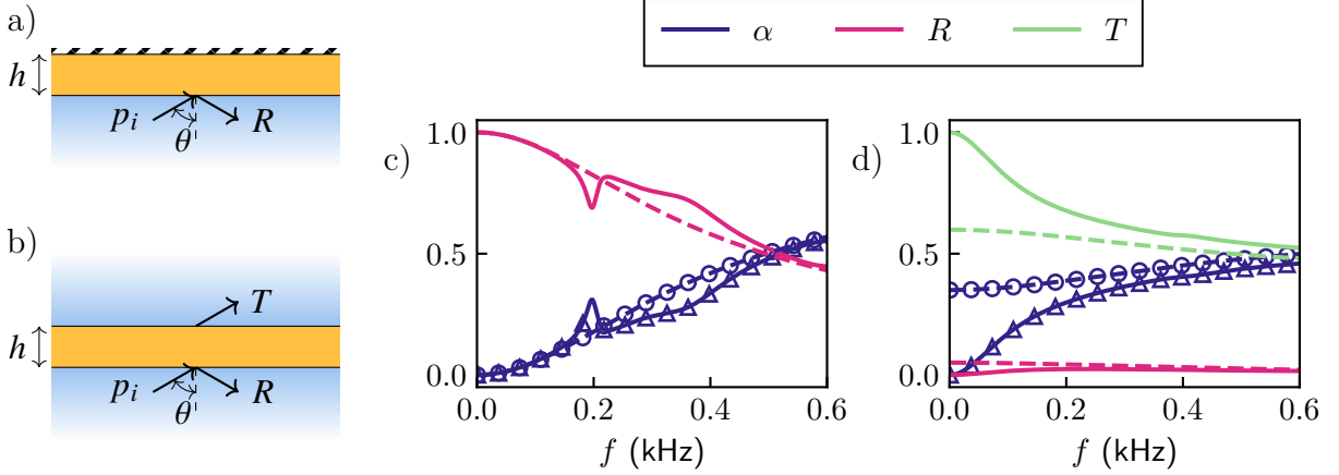
Fig. 1.1: Diagram for the a) reflection, b) transmission problem. Scattering coefficients from a poroelastic layer (continuous) and equivalent fluid layer (dashed) computed using the GM for the c) reflection, d) transmission problem. Results computed with the TMM are also shown for the absorption coefficient for the equivalent fluid ( \circ ) and for the absorption coefficient ( \Delta )
