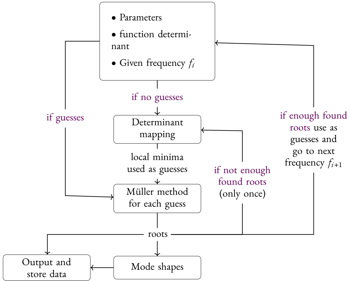
Fig. 1.6: Description of the routine
