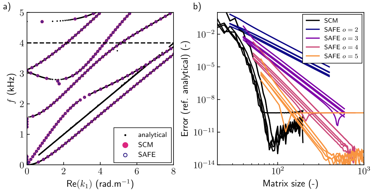
Fig. 1.4: a) Dispersion relation for the Lamb modes with the root-finding results, alongside the spectral collocation and semi-analytical finite elements solutions. b) Convergence curve of the 2 methods at a given frequency f = 4 kHz. The multiple lines depicts the convergence of each wavenumber.
