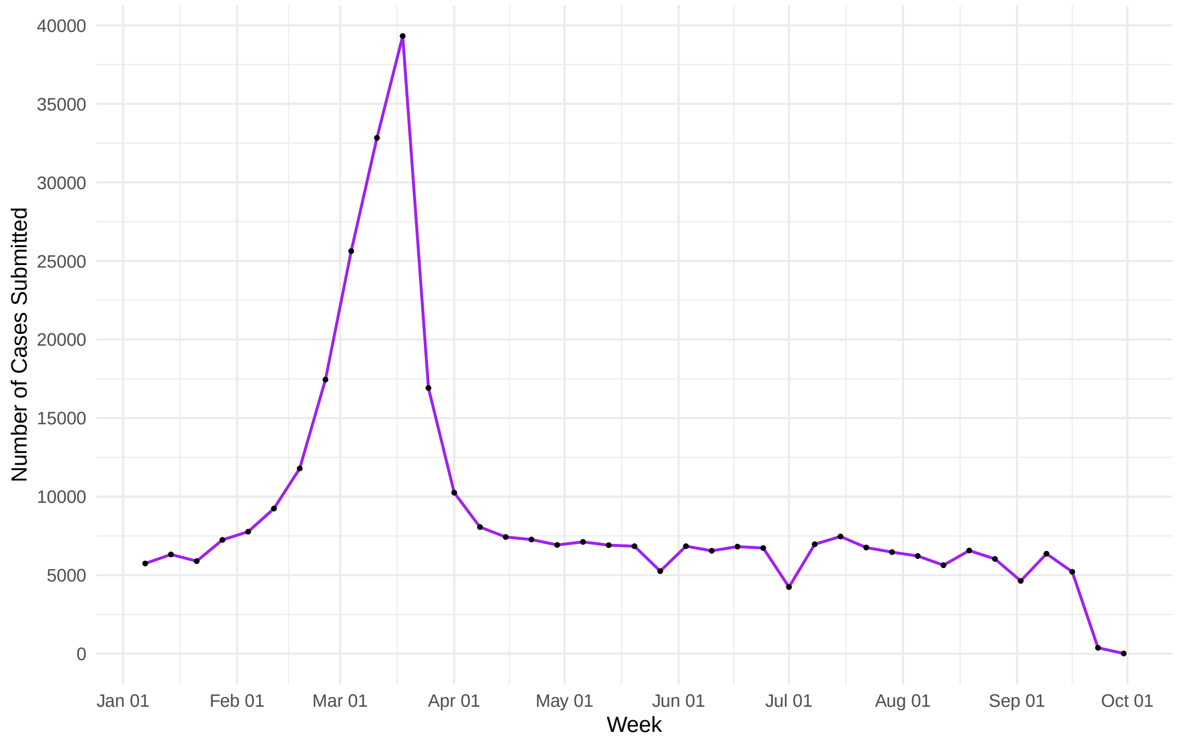
Weekly H-1B Cases Submitted in 2013
