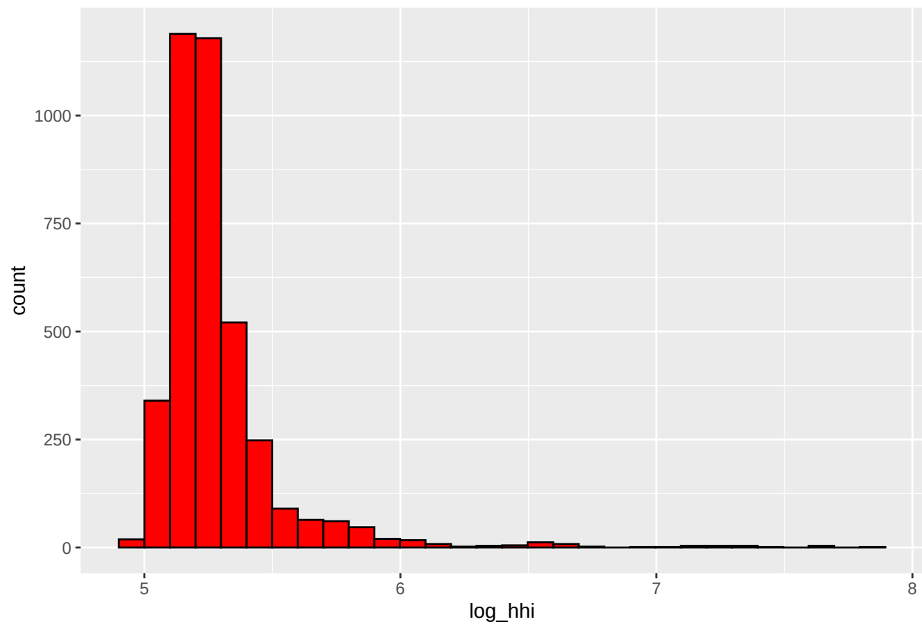
Distribution of \log(\text{HHI})
