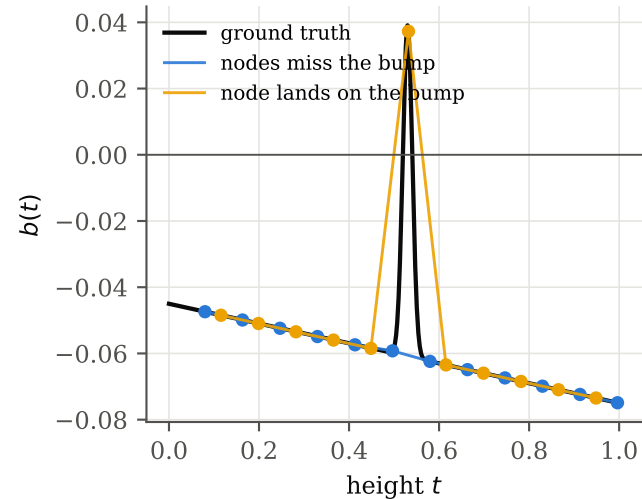
(a) sampling butchers a narrow feature: visibility depends on node phase
