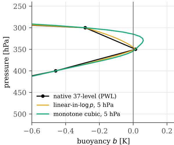
(b) issue-77 column, reconstructed: the bump is real but reconstruction-dependent
