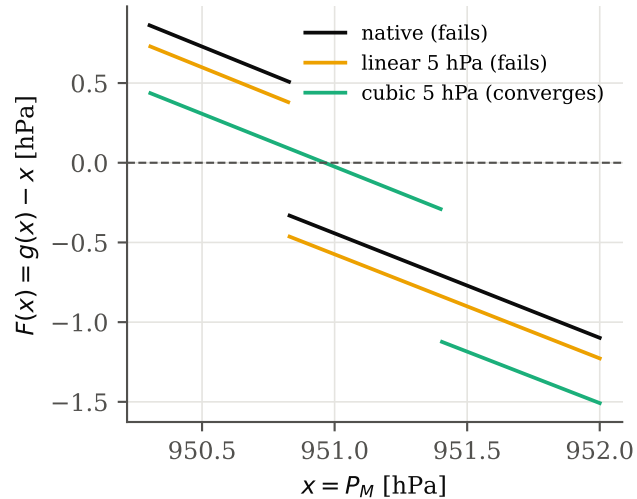
(c) recovery moves the gap but cannot remove it: zero crossing vs gap position
