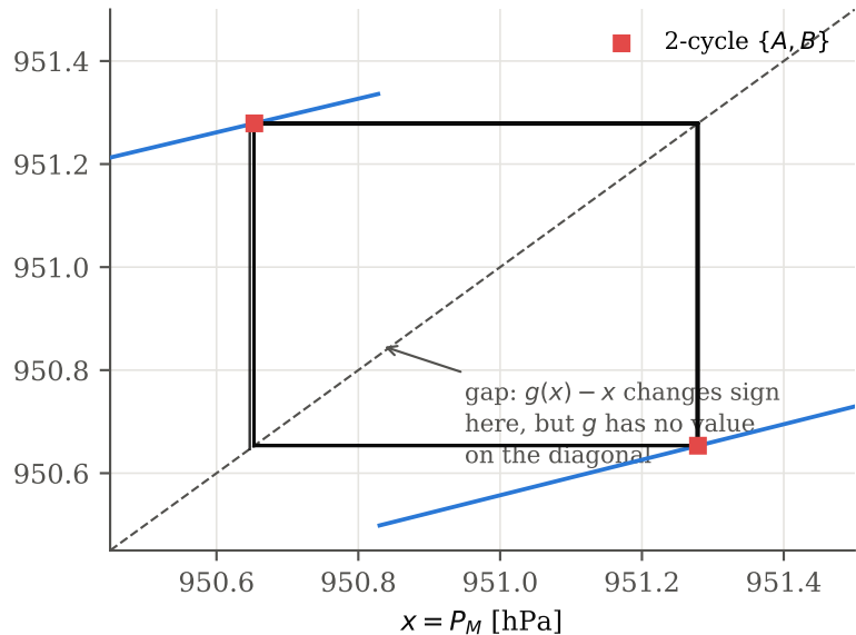
(b) zoom: the diagonal crosses inside the gap
