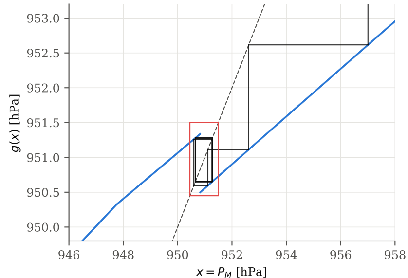
(a) issue-77 column: the map g
