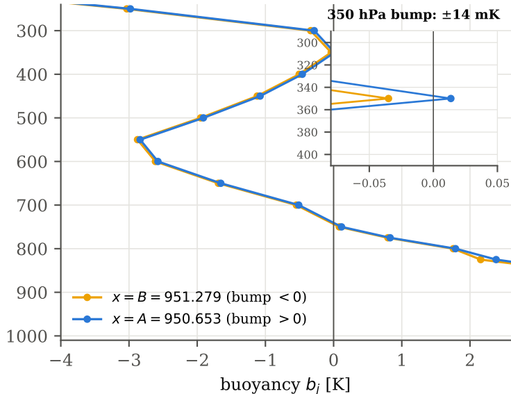
(a) eyewall-parcel buoyancy at the two phases
