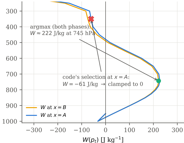
(b) work integral and the two selections
