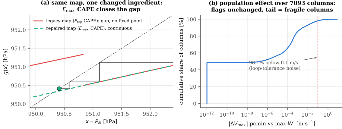
Figure 12: The repair: the same map (2) evaluated with the two CAPE conventions on the Francine column. (a) With the legacy E_{\text{top}} (red, solid) the map has the gap and no fixed point. With E_{\text{max}} (teal, dashed) it is continuous, crosses the diagonal, and the iteration converges (dot). On the right branch the two coincide to line width — red shows through the dash gaps — because there the topmost-positive level already selects the dominant lower cell; on the left branch they differ by the full effect of the 222 \text{ J kg}^{-1} clamp. (b) Cumulative distribution of |\Delta V_{\text{max}}| between conventions over the benchmark: 39% bit-identical (left edge, clipped to 10^{-12} ), 98.1% below 0.1 \text{ m s}^{-1} , and a 1.9% tail of discontinuity-adjacent columns.
