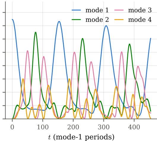
(b) \alpha -FPUT ( \alpha = 1/4 ): mixing + recurrence
