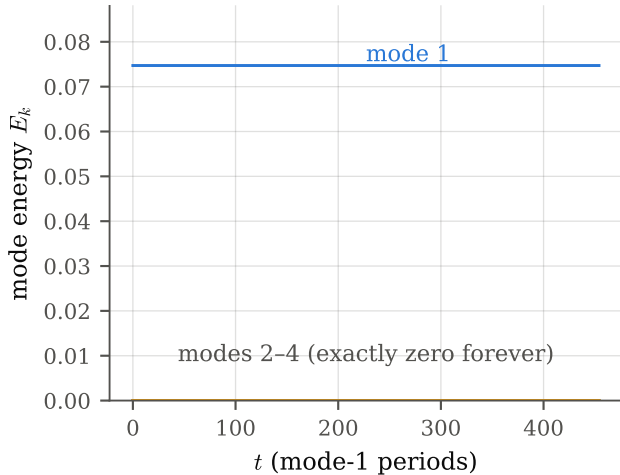
(a) harmonic ( \alpha = 0 ): integrable, frozen
