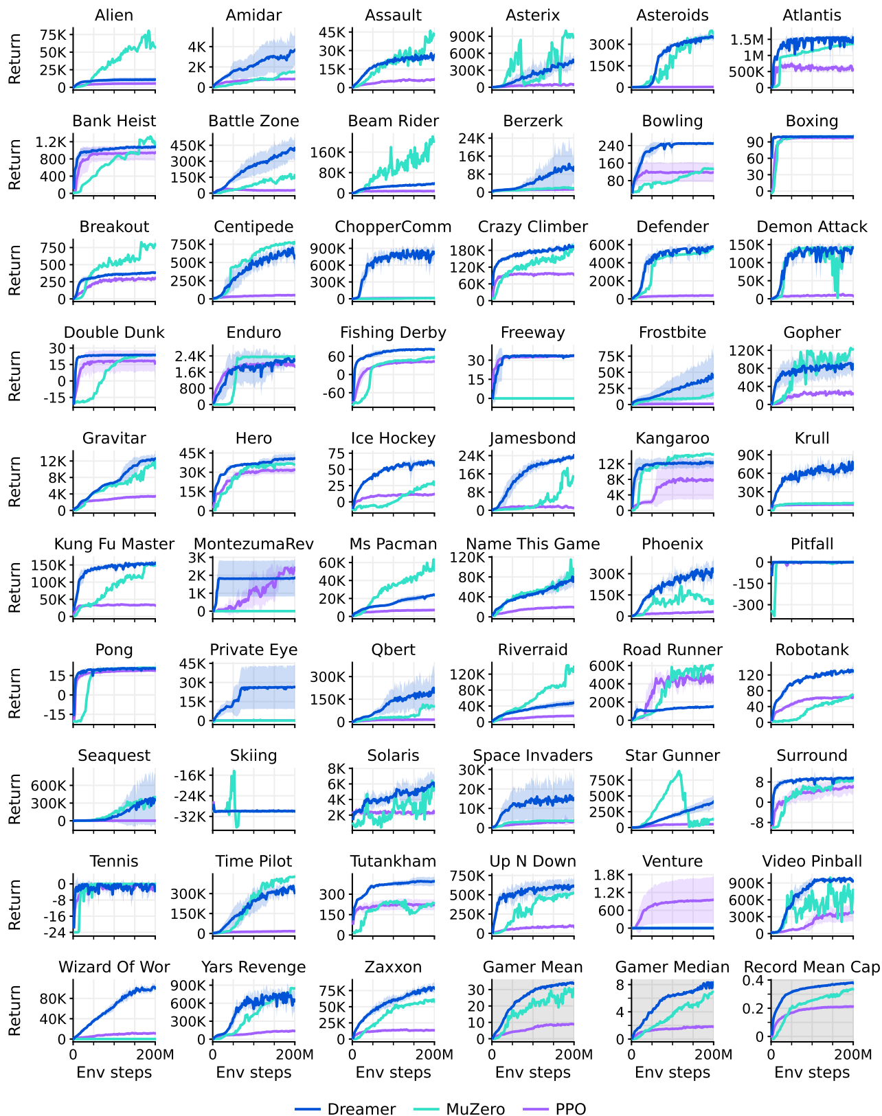
Figure 10: Atari learning curves.
