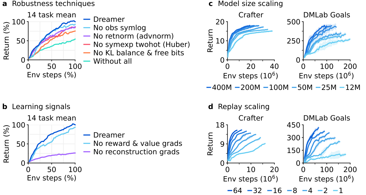
Figure 6: Ablations and robust scaling of Dreamer. a , All individual robustness techniques contribute to the performance of Dreamer on average, although each individual technique may only affect some tasks. Training curves of individual tasks are included in the supplementary material. b , The performance of Dreamer predominantly rests on the unsupervised reconstruction loss of its world model, unlike most prior algorithms that rely predominantly on reward and value prediction gradients 7,5,8 . c , The performance of Dreamer increases monotonically with larger model sizes, ranging from 12M to 400M parameters. Notably, larger models not only increase task performance but also require less environment interaction. d , Higher replay ratios predictably increase the performance of Dreamer. Together with model size, this allows practitioners to improve task performance and data-efficiency by employing more computational resources.
