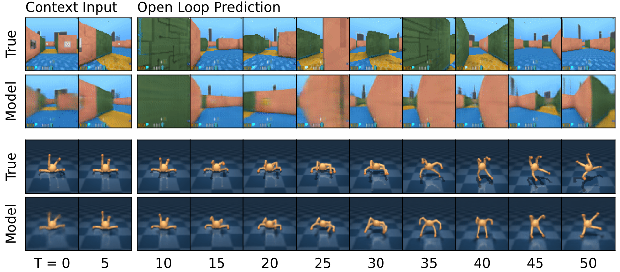
Figure 4: Multi-step video predictions of a DMLab maze (top) and a quadrupedal robot (bottom). Given 5 context images and the full action sequence, the model predicts 45 frames into the future without access to intermediate images. The world model learns an understanding of the underlying structure of each environment.
