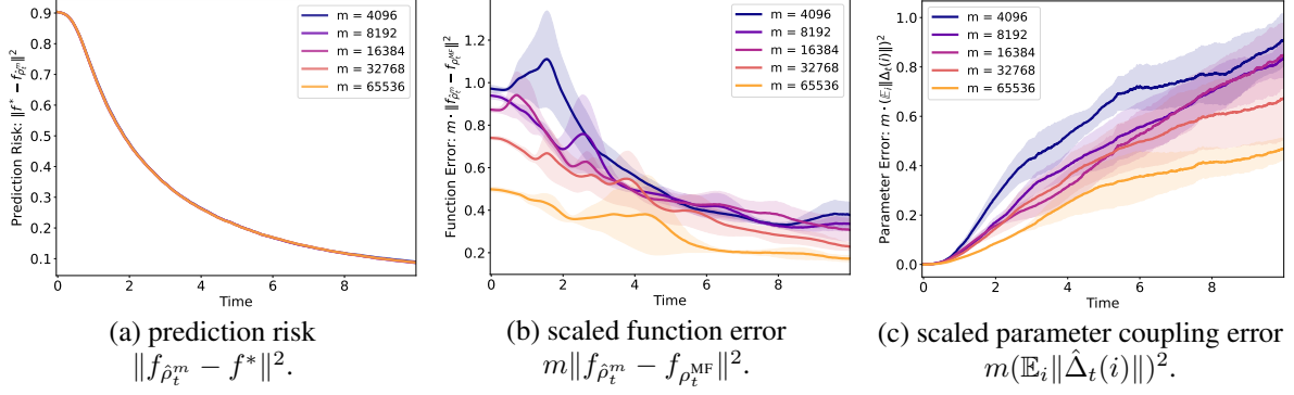
Figure 3: Well-specified single-index target function f^*(x) = \text{He}_4(x^\top w^*) , x \sim \mathcal{N}(0, I_d) , and \sigma = \text{He}_4 . We set d = 32 and learning rate \eta = 0.005 .
