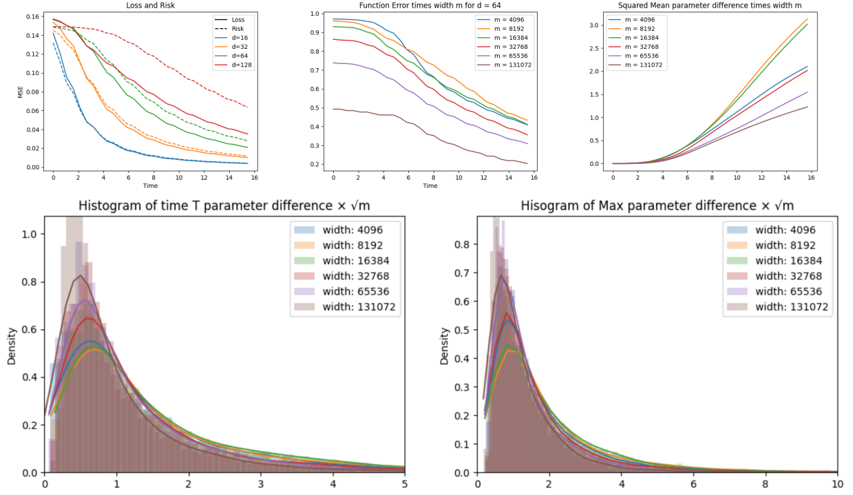
Figure 9: \text{Random}_{8,8} ( d = 64 ). Top left: Loss/Risk. Top Middle: Function error m\|f_{\hat{\rho}_t^n} - f_{\rho_t^{\text{MF}}}\|^2 Top right: Parameter error m\left(\mathbb{E}_i\|\hat{\Delta}_t(i)\|\right)^2 . Bottom left: histogram of \mathbb{E}_i\delta_{\sqrt{m}\|\hat{\Delta}_t(i)\|} at t = T = 16 . Bottom right: histogram of \mathbb{E}_i\delta_{\max_{t \leq T} \sqrt{m}\|\hat{\Delta}_t(i)\|} .
