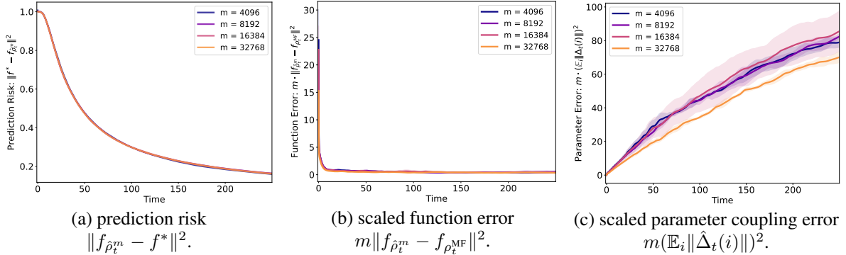
Figure 5: 4-parity target function f^*(x) = \prod_{j \leq 4} [x]_j , [x]_i \sim \text{Unif}\{1, -1\} , and \sigma = \text{SoftPlus} with temperature 16. We set d = 64 and learning rate \eta = 0.05 .
