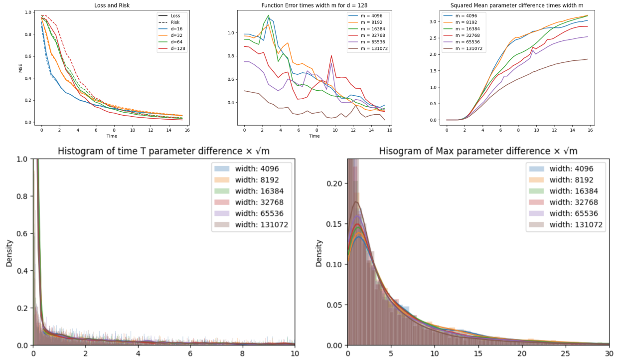
Figure 7: \text{He}_4 ( d = 128 ) Top left: Loss/Risk. Top Middle: Function error m\|f_{\hat{\rho}_t^m} - f_{\rho_t^{\text{MF}}}\|^2 Top right: Parameter error m\left(\mathbb{E}_i\|\hat{\Delta}_t(i)\|\right)^2 . Bottom left: histogram of \mathbb{E}_i\delta_{\sqrt{m}\|\hat{\Delta}_t(i)\|} at t = T = 16 . Bottom right: histogram of \mathbb{E}_i\delta_{\max_{t \leq T} \sqrt{m}\|\hat{\Delta}_t(i)\|} .
