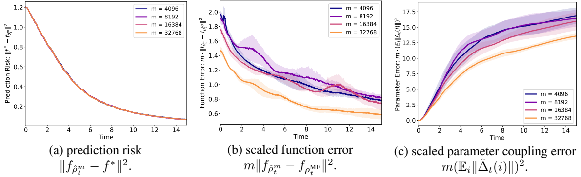
Figure 4: Mis-specified single-index target function f^*(x) = 0.8\text{He}_4(x^\top w^*) + 0.6\text{He}_6(x^\top w^*) , x \sim \mathcal{N}(0, I_d) , and \sigma = \text{He}_4 + \text{He}_6 . We set d = 32 and learning rate \eta = 0.005 .
