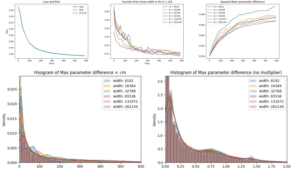
Figure 10: Staircase ( d = 128 ) Top left: Loss/Risk. Top Middle: Function error m\|f_{\hat{\rho}_t^m} - f_{\rho_t^{\text{MF}}}\|^2 Top right: Unscaled parameter error \left(\mathbb{E}_i\|\hat{\Delta}_t(i)\|\right)^2 . Bottom left: histogram of \mathbb{E}_i\delta_{\max_{t \leq T} \sqrt{m}\|\hat{\Delta}_t(i)\|} . Bottom right: histogram of \mathbb{E}_i\delta_{\max_{t \leq T} \|\hat{\Delta}_t(i)\|} .
