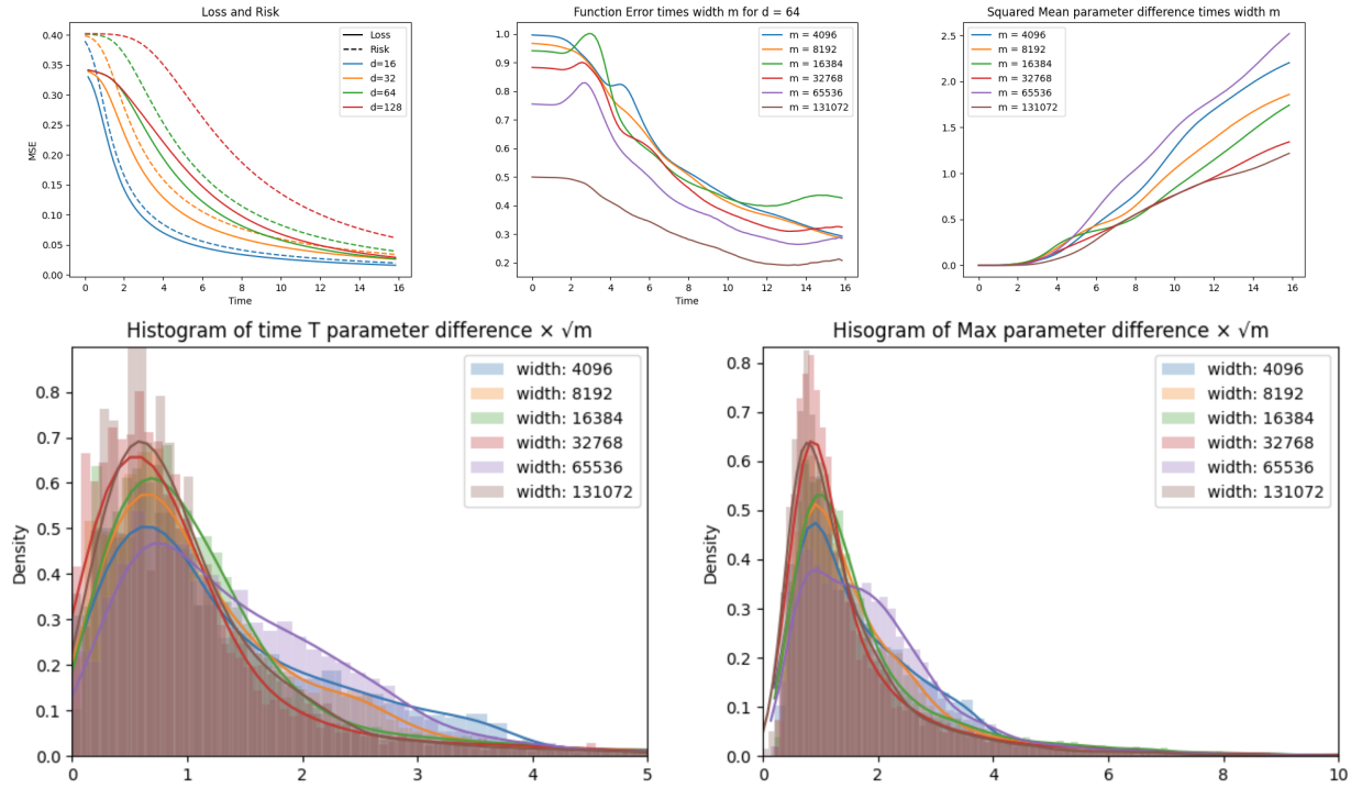
Figure 8: Circle ( d = 64 ) Top left: Loss/Risk. Top Middle: Function error m\|f_{\hat{\rho}_t^m} - f_{\rho_t^{\text{MF}}}\|^2 Top right: Parameter error m\left(\mathbb{E}_i\|\hat{\Delta}_t(i)\|\right)^2 . Bottom left: histogram of \mathbb{E}_i\delta_{\sqrt{m}\|\hat{\Delta}_t(i)\|} at t = T = 16 . Bottom right: histogram of \mathbb{E}_i\delta_{\max_{t \leq T} \sqrt{m}\|\hat{\Delta}_t(i)\|} .
