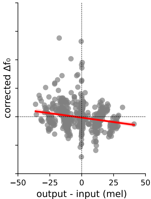
speech-like vocalizations
