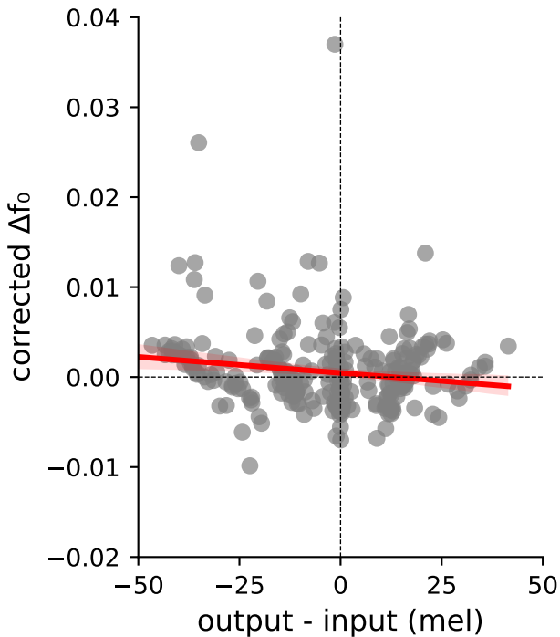
other vocalizations
