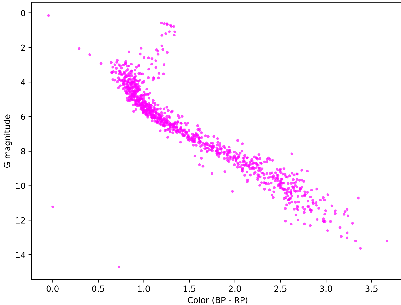
Color-Magnitude Diagram (CMD) - Gaia DR3
