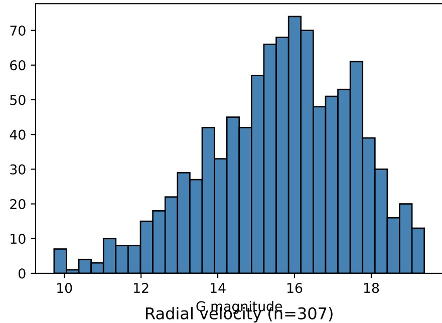
Magnitude distribution
