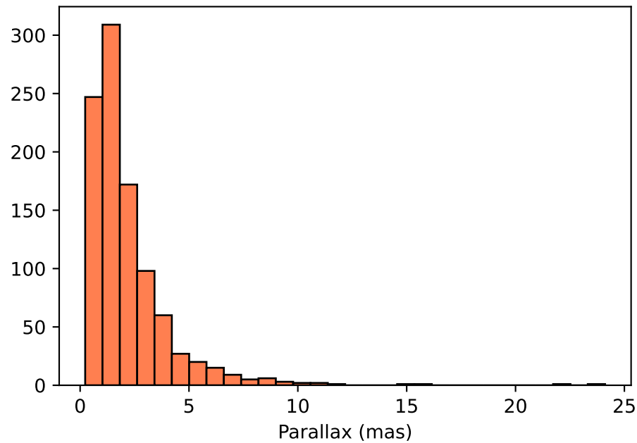
Parallax distribution
