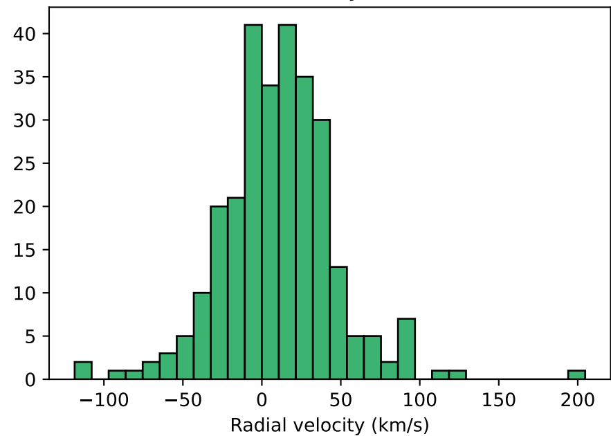
Radial velocity (n=281)
